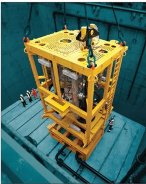
A helico-axial multiphase boosting pump jointly developed with Sulzer Pumps undergoing testing.
